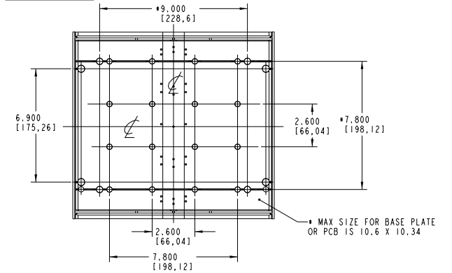
CLLPH-325
